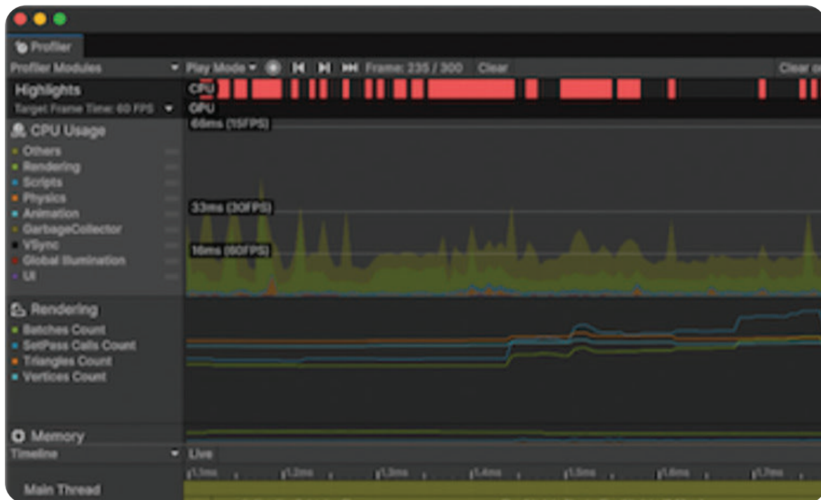
Gambar 6.2 Contoh Program Profiler Sumber: Unity (2024)
